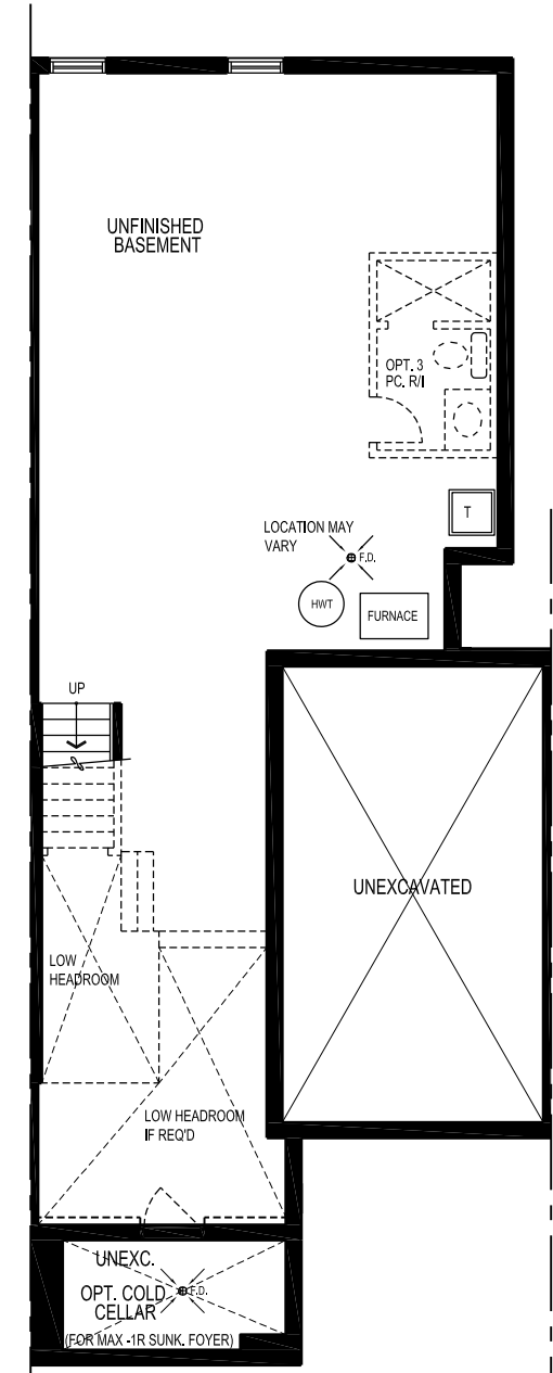
BASEMENT PLAN
