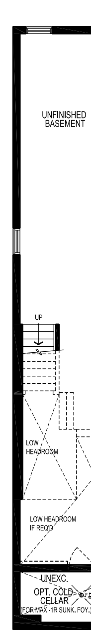
BASEMENT PLAN END CONDITION
